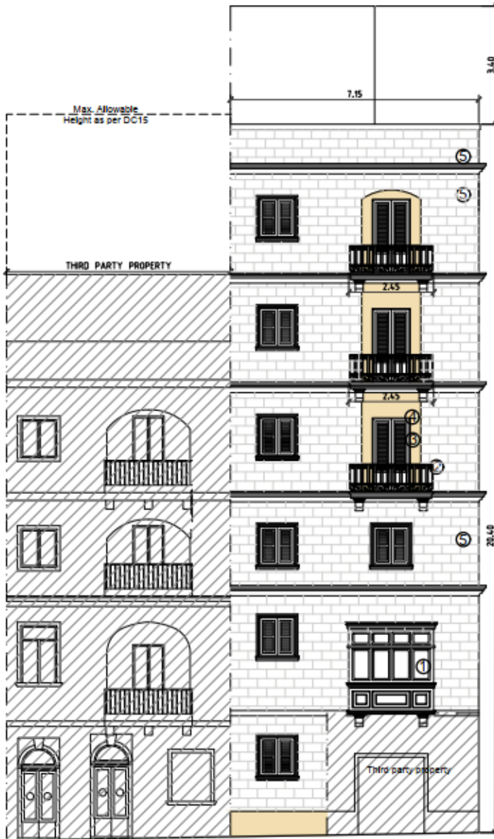
02 ELEVATION IN TRIQ SIR W. REID ELEVATION_AS PROPOSED SCALE 1:100
