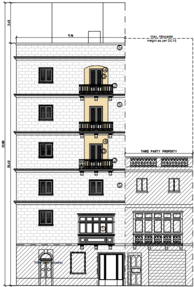
01 ELEVATION IN TRIQ C. MANCHE ELEVATION_AS PROPOSED SCALE 1:100
