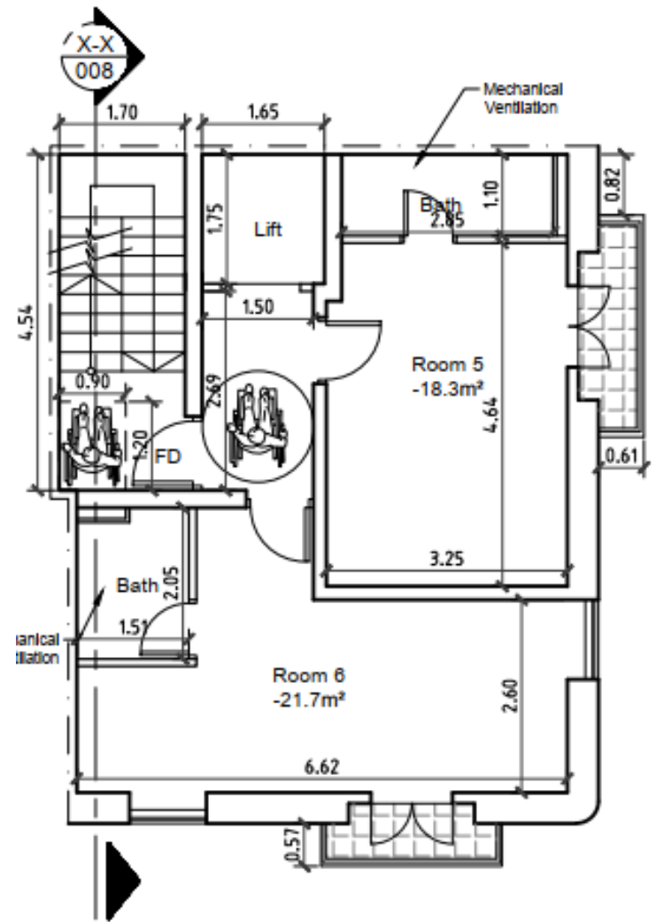
03 THIRD FLOOR PLAN -- PLAN_AS PROPOSED SCALE 1:100
