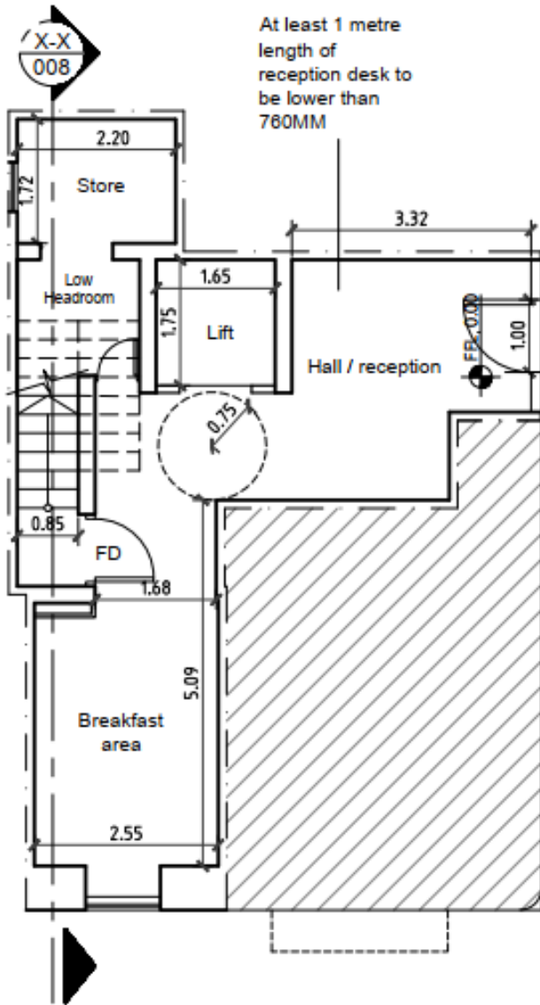
04 GROUND FLOOR PLAN PLAN_AS PROPOSED SCALE 1:100
