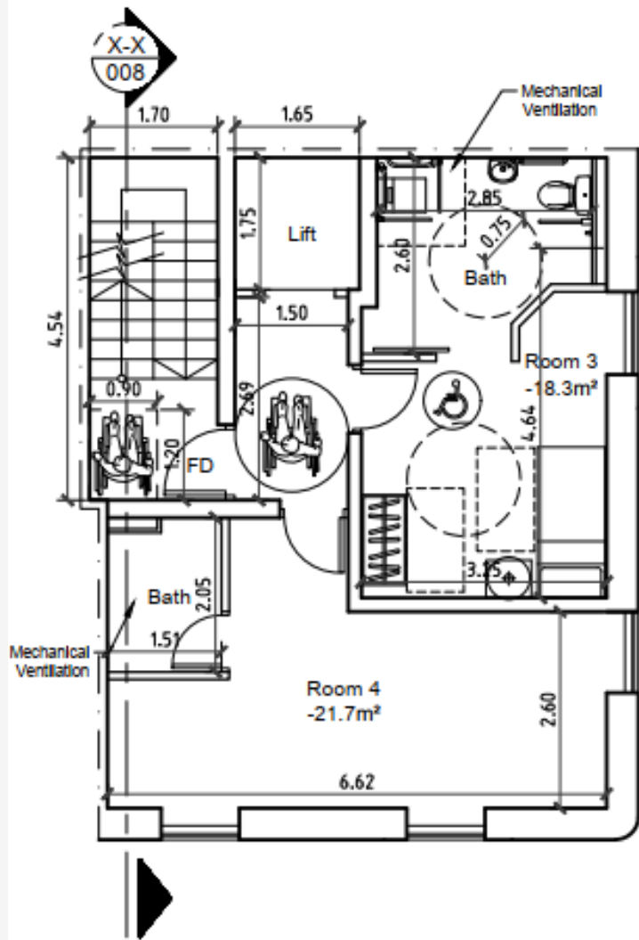
03 SECOND FLOOR PLAN -- PLAN_AS PROPOSED SCALE 1:100
