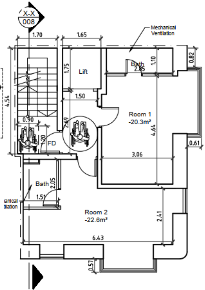
03 FIRST FLOOR PLAN PLAN_AS PROPOSED SCALE 1:100
